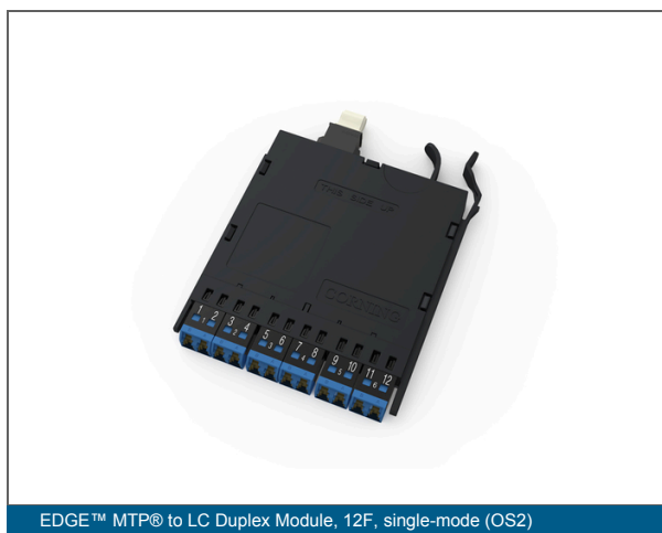
EDGE™ MTP® to LC Duplex Module, 12F, single-mode (OS2)
